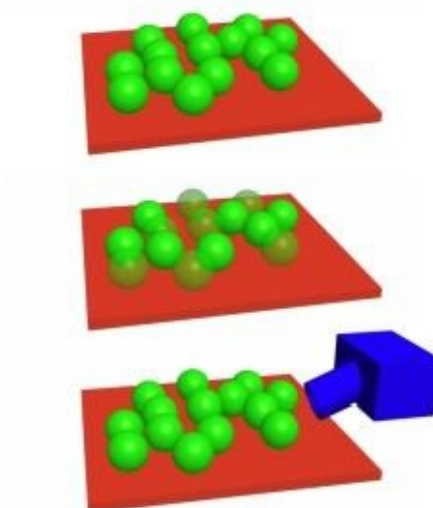
Quantum Zeno effect
