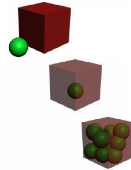
Quantum superposition
