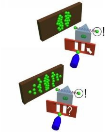
Quantum superposition
