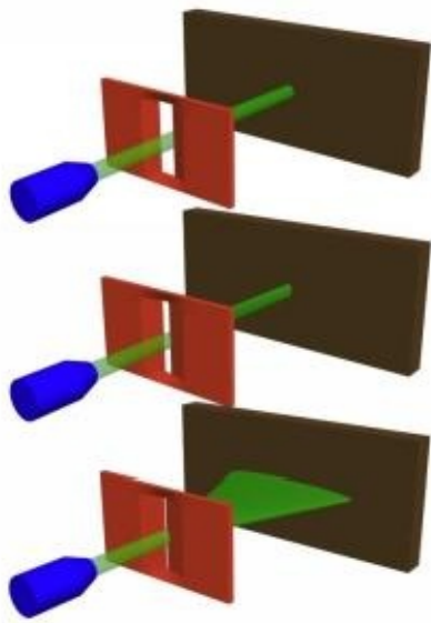
Meissner effect
